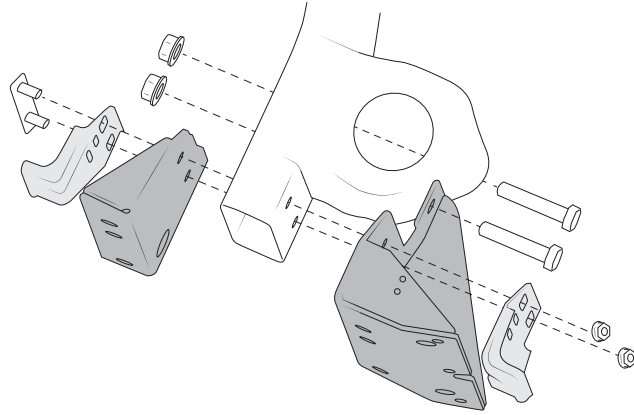
Figure 14-A: With Factory Compatibility Beam and Hardware (Left Side) Kit: 10308002
